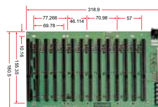
14-slot Passive ISA Backplane
