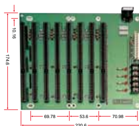
8-slot Passive ISA Backplane
