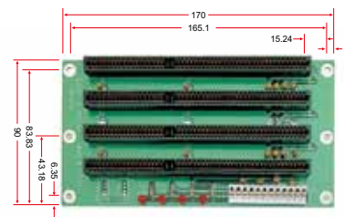
4-slot Passive ISA Backplane
