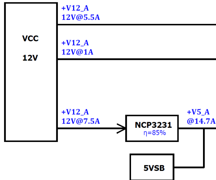
Figure 2 PCOM-B657VGL Power on sequence
