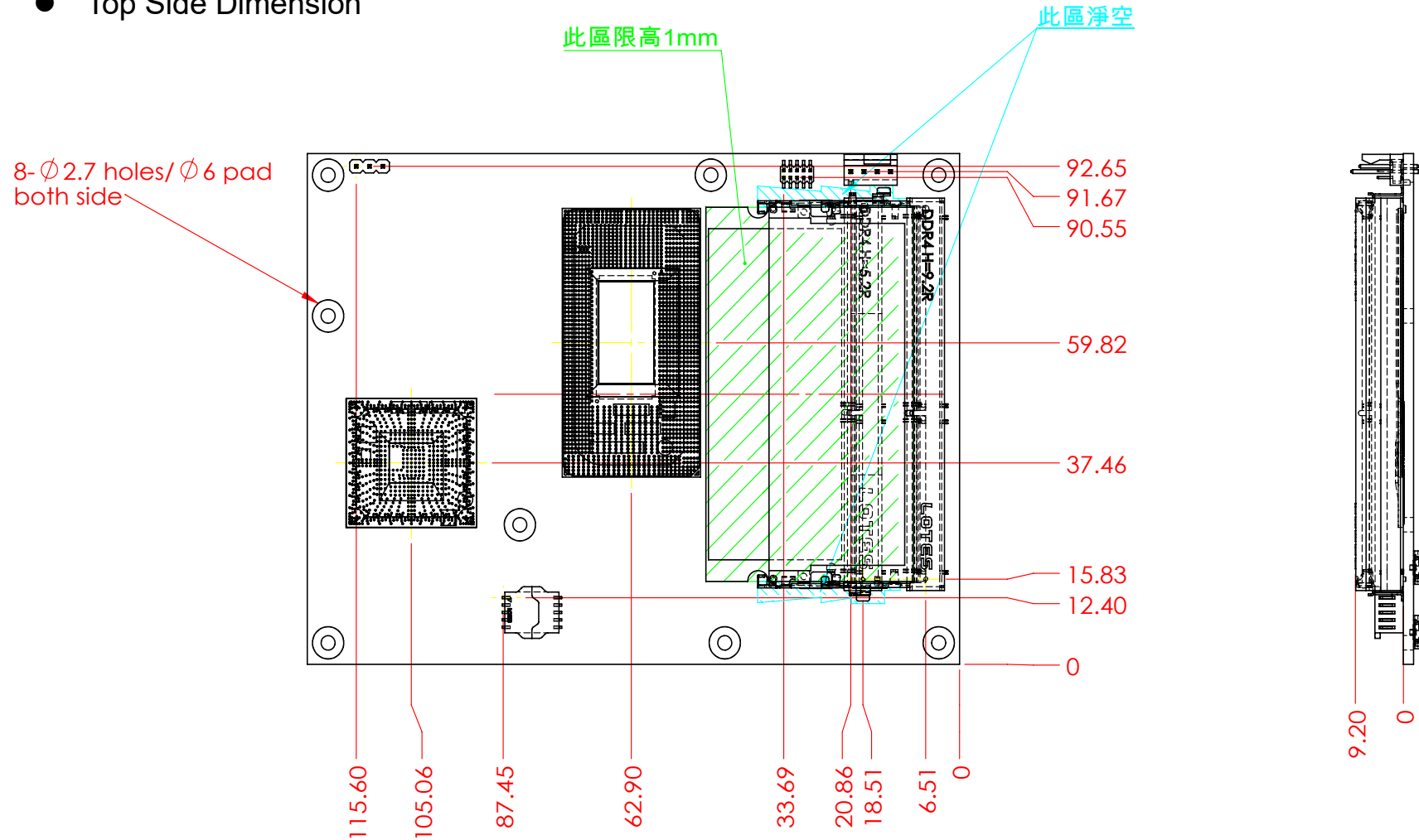
Figure 6 Mechanical Dimension - Top
